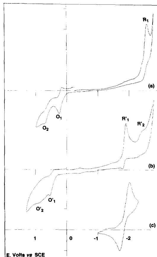
Fig. 2. Cyclic voltammograms of complexes [Ni_2(CO)_3(dppm)_2] and 2 (2 mM in THF, 0.3 M n-Bu_4NBF_4 , 20°C) at a gold disk electrode (diameter 0.5 mm): (a) complex [Ni_2(CO)_3(dppm)_2] ( 0.2 V s^{-1} ); (b) complex 2 ( 0.2 V s^{-1} ); (c) complex 2 ( 5 V s^{-1} ).
