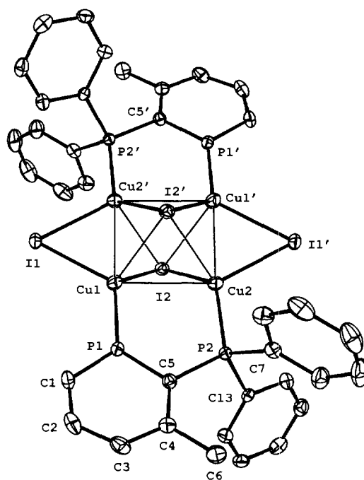
Fig. 3. ORTEP drawing of the molecular structure of complex [\text{Cu}_4(\mu\text{-I})_2(\mu\text{-I})_2] ( 3 ) as determined by single crystal X-ray diffraction study with the atomic labelling scheme. Ellipsoids are scaled to enclose 50% of the electron density. Hydrogen atoms are omitted for clarity.
